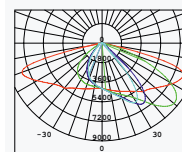
Lumileds LED 120W 15955lm Clear Glass 155° Class I, IP65
